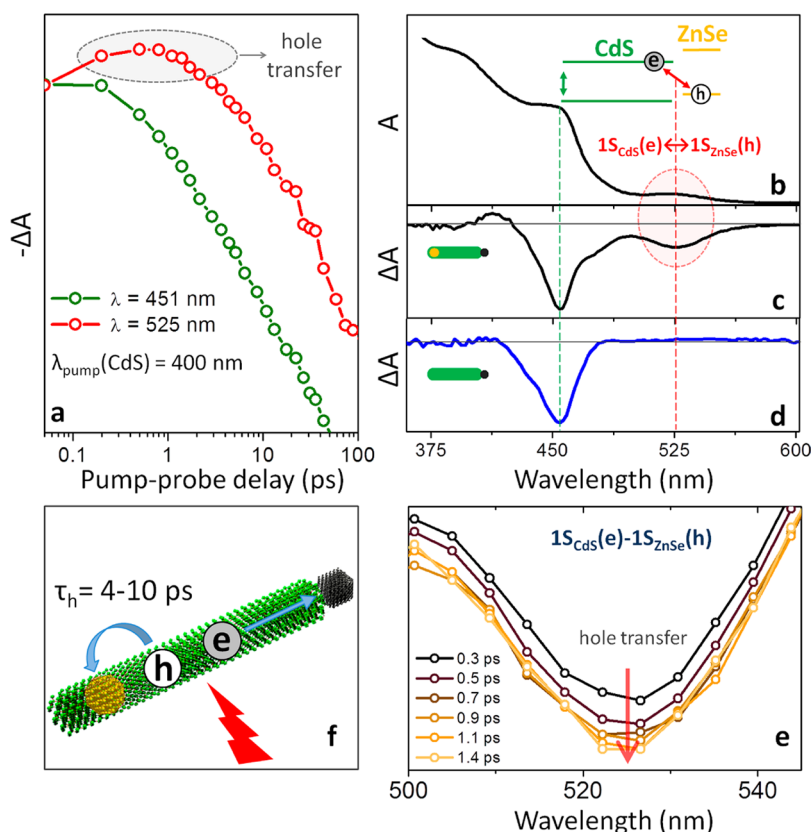
Figure 4. (a) Recovery of the TA bleach for the two spectral bands in ZnSe/CdS/Pt nanorods associated with 1S_h(\text{CdS}) \rightarrow 1S_e(\text{CdS}) (green curve) and 1S_h(\text{ZnSe}) \rightarrow 1S_e(\text{CdS}) (red curve) transitions. (b) Steady state absorption spectra of ZnSe/CdS/Pt heteronanocrystals showing the onset of spatially indirect absorbing transition, 1S_h(\text{ZnSe}) \rightarrow 1S_e(\text{CdS}) . (c) TA spectra of ZnSe/CdS/Pt nanorods highlighting the 1S_h(\text{ZnSe}) \rightarrow 1S_e(\text{CdS}) bleach near \lambda = 525 nm. (d) TA spectra confirming the lack of the spatially indirect 1S_h(\text{ZnSe}) \rightarrow 1S_e(\text{CdS}) bleach in single-phase CdS nanorods appended with a Pt tip. (e) Temporal evolution of the TA bleach centered near the 1S_h(\text{ZnSe}) \rightarrow 1S_e(\text{CdS}) transition. The early time increase in the bleach strength is attributed to a hole transfer from CdS into ZnSe (see text). (f) Schematic representation of the hole transfer process in ZnSe/CdS/Pt heteronanocrystals.
